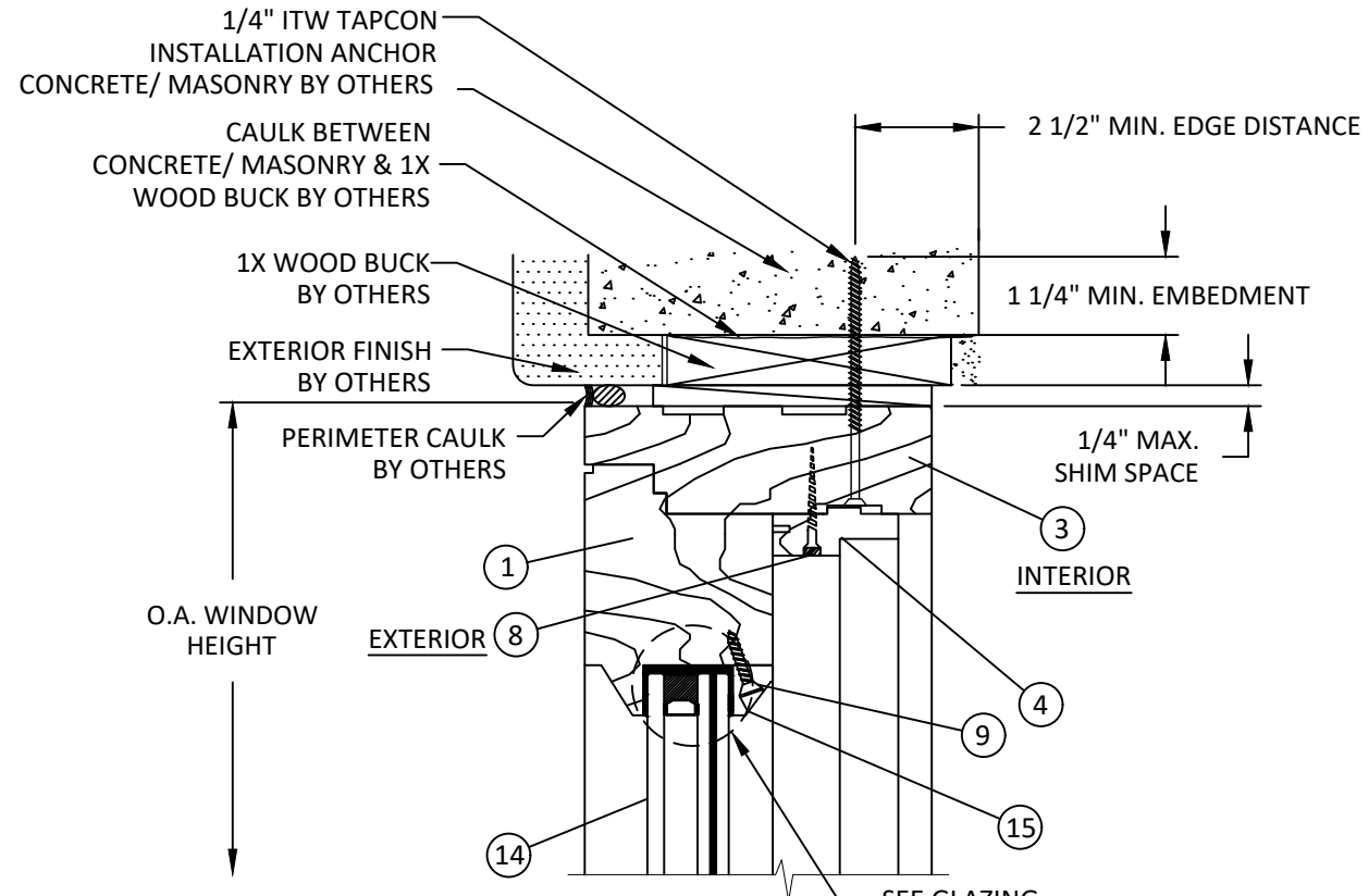
C 4 VERTICAL SECTION HEAD - CONCRETE/MASONRY
