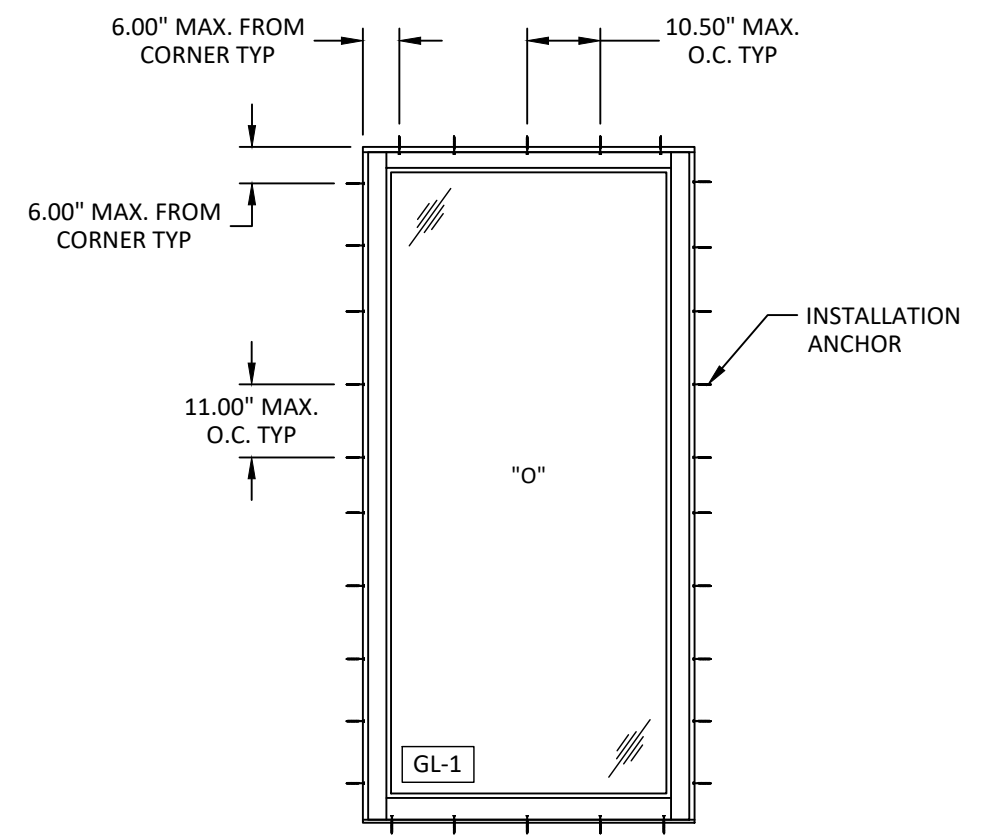
ANCHOR LAYOUT
