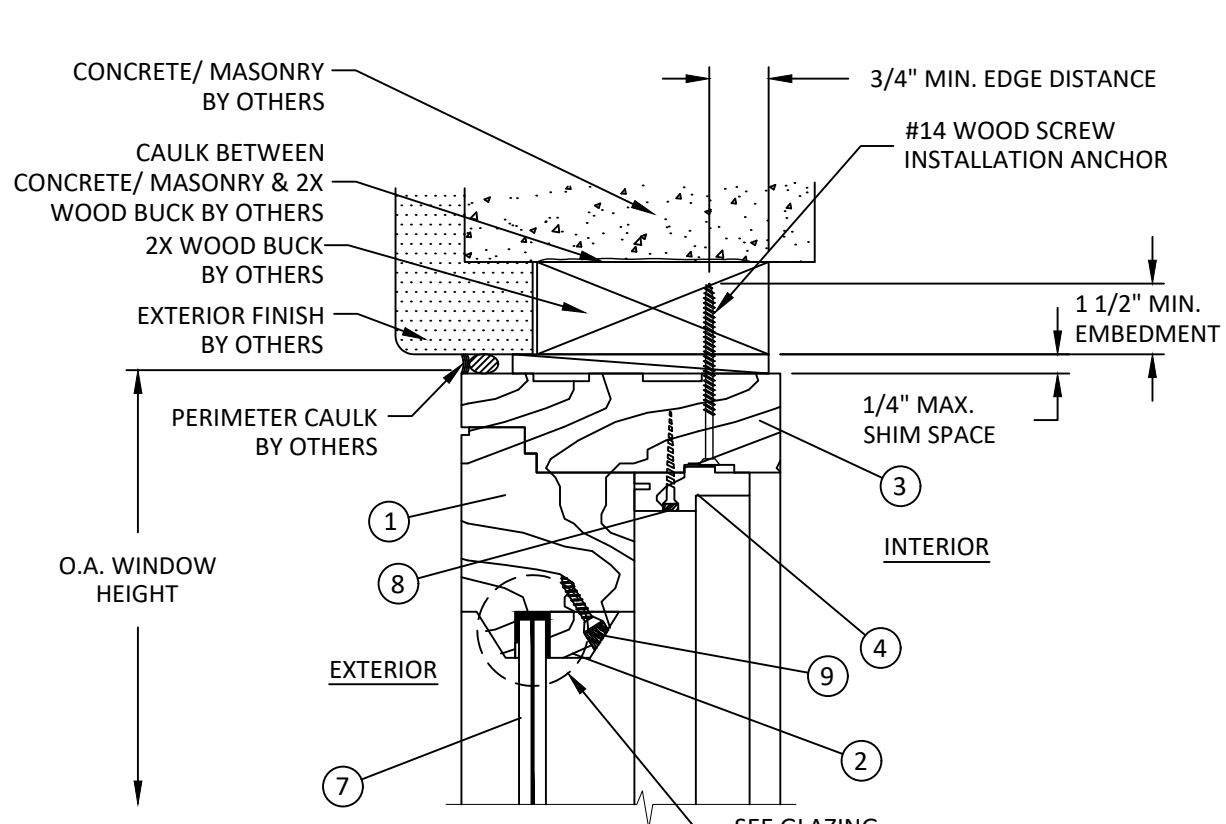
A 4 VERTICAL SECTION HEAD - 2X WOOD BUCK
