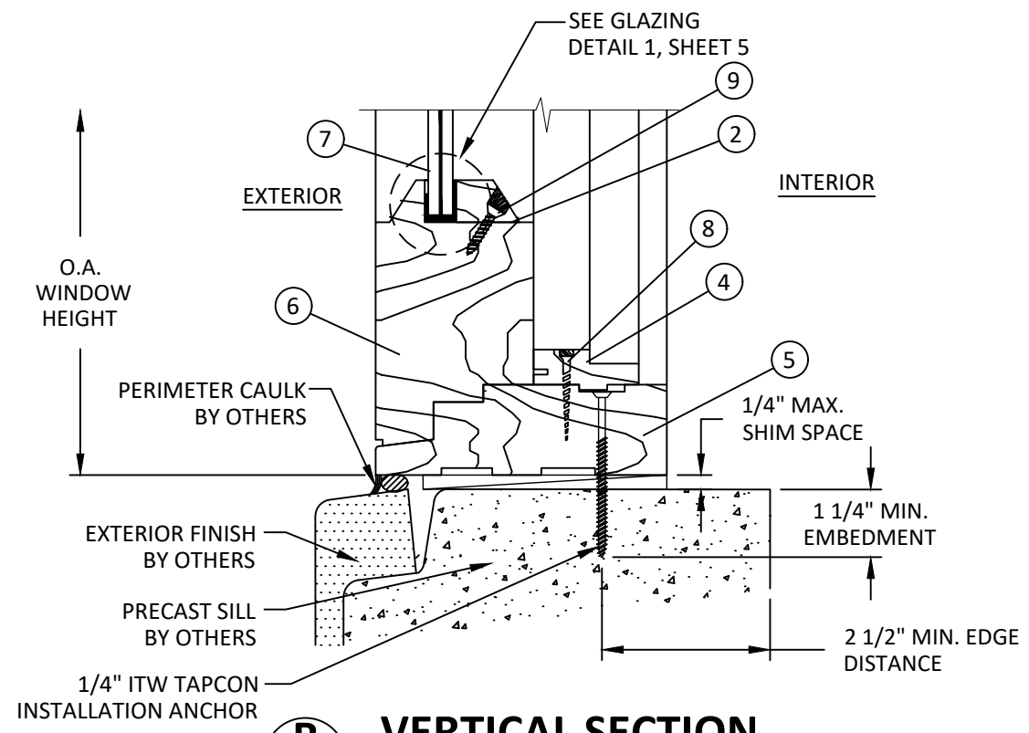
B 4 VERTICAL SECTION SILL - CONCRETE/MASONRY PRE-CAST SILL
