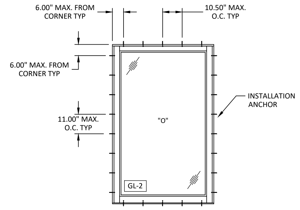
ANCHOR LAYOUT
