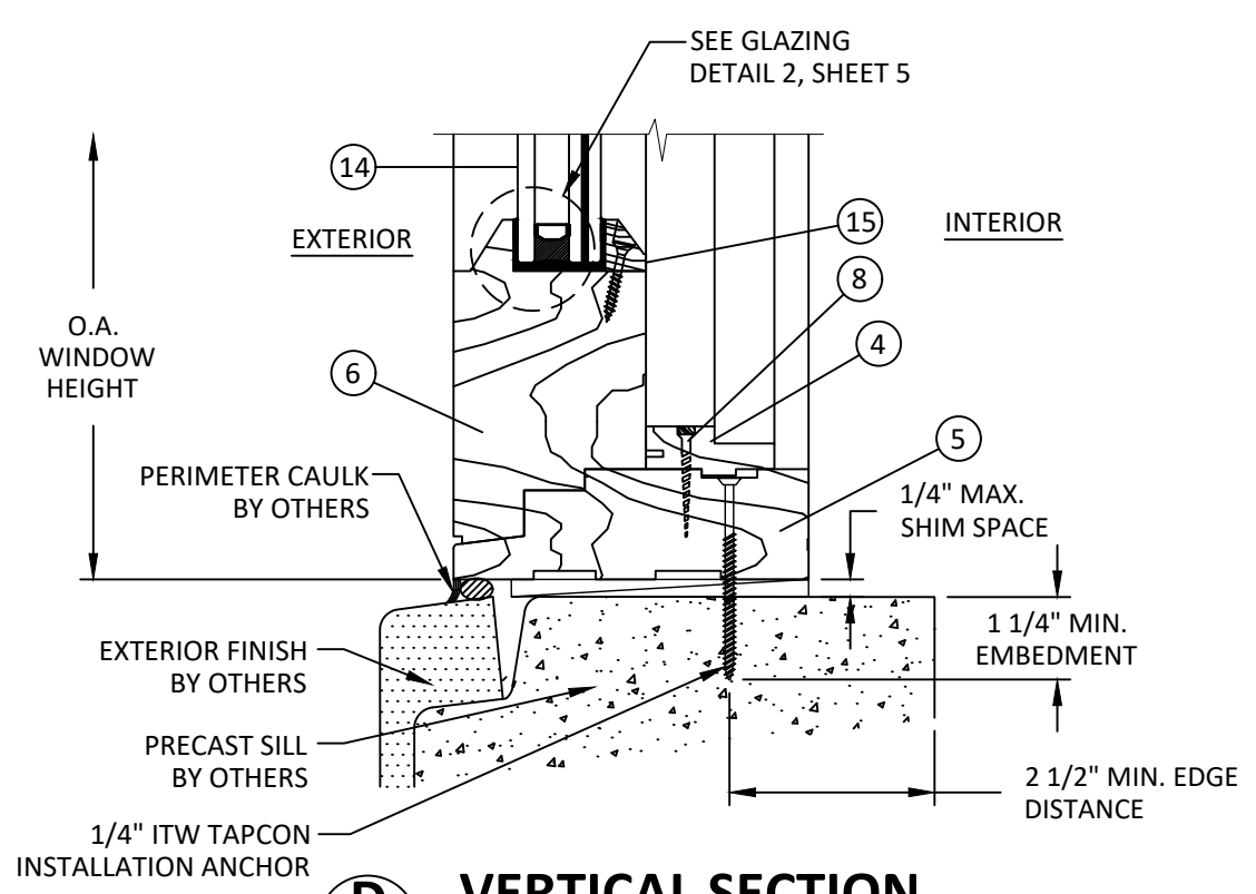
D 4 VERTICAL SECTION SILL - CONCRETE/MASONRY PRE-CAST SILL
