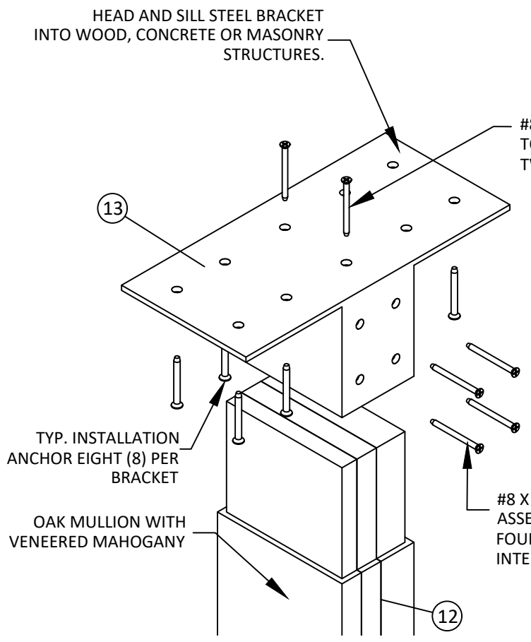
MULLION BRACKET ASSEMBLY
